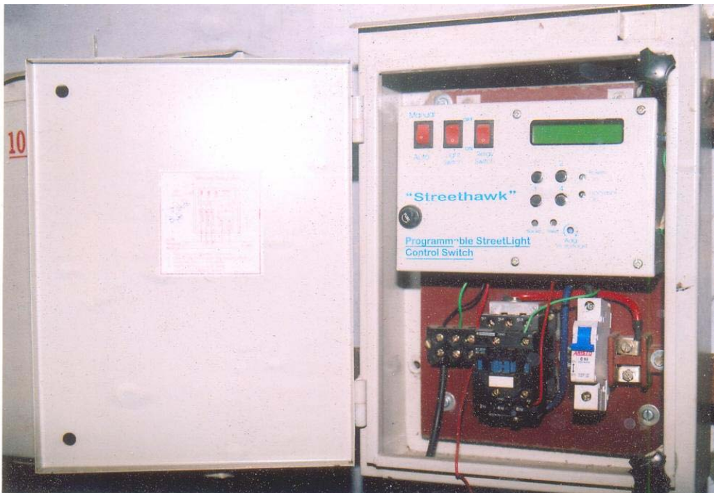
Microprocessor controlled Street Light Timer Switch
