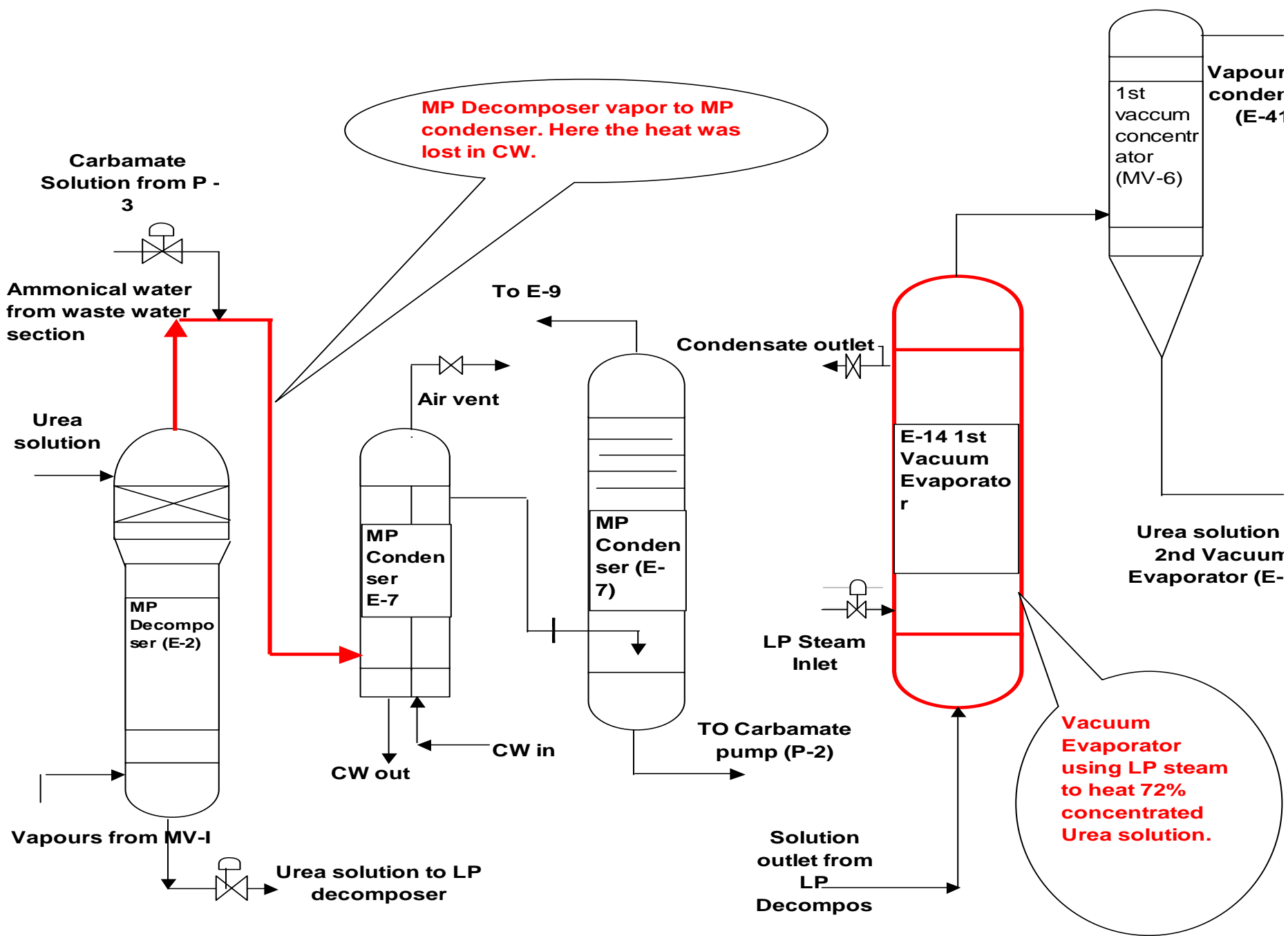
ORIGINAL SCHEME (WITHOUT PRECONCENTRATOR) IN UREA PLANT
