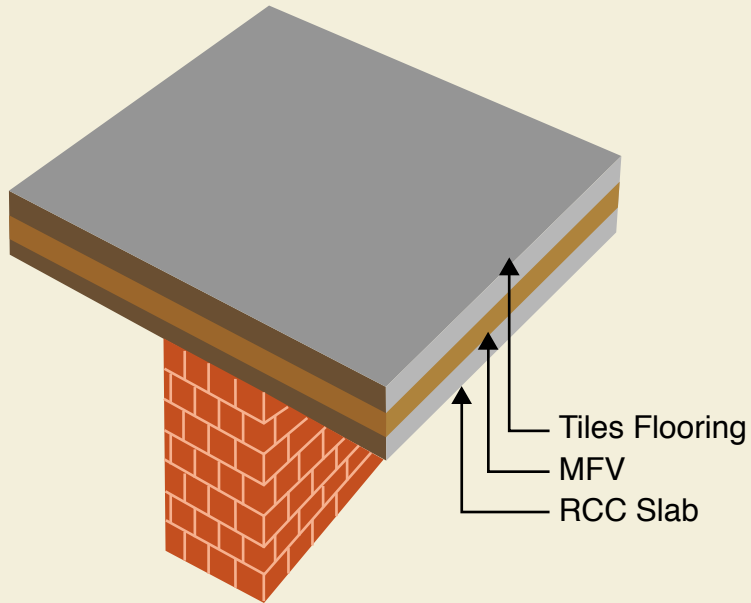
Insulation with RCC Slab
