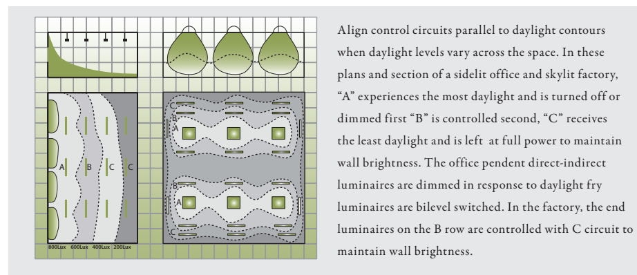
Fig. 12: Plan Views of Daylight Isolux Contours (Source: Advanced Lighting Guidelines, New Buildings Institute)
